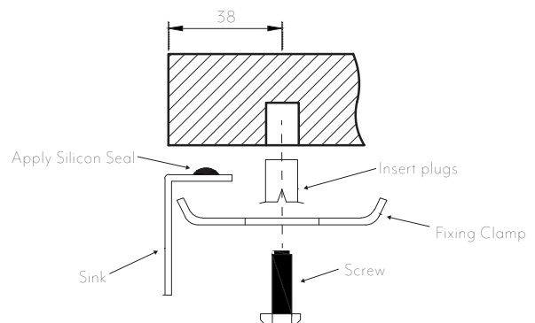
UNDERMOUNT INSTALLATION
