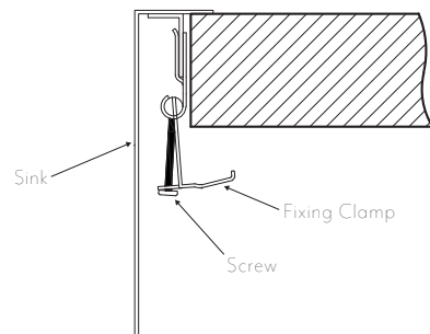
TOP MOUNT INSTALLATION
