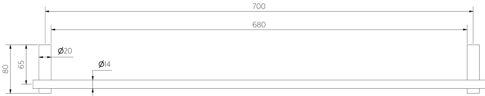
Top View
