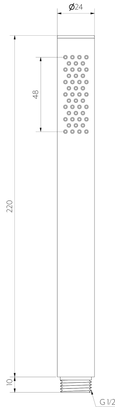
Hand Shower Front View
