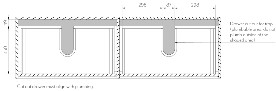
Section K-K
