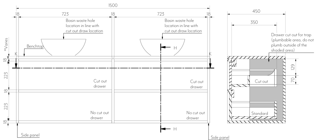
Section K-K
