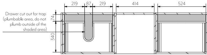
Section B-B
